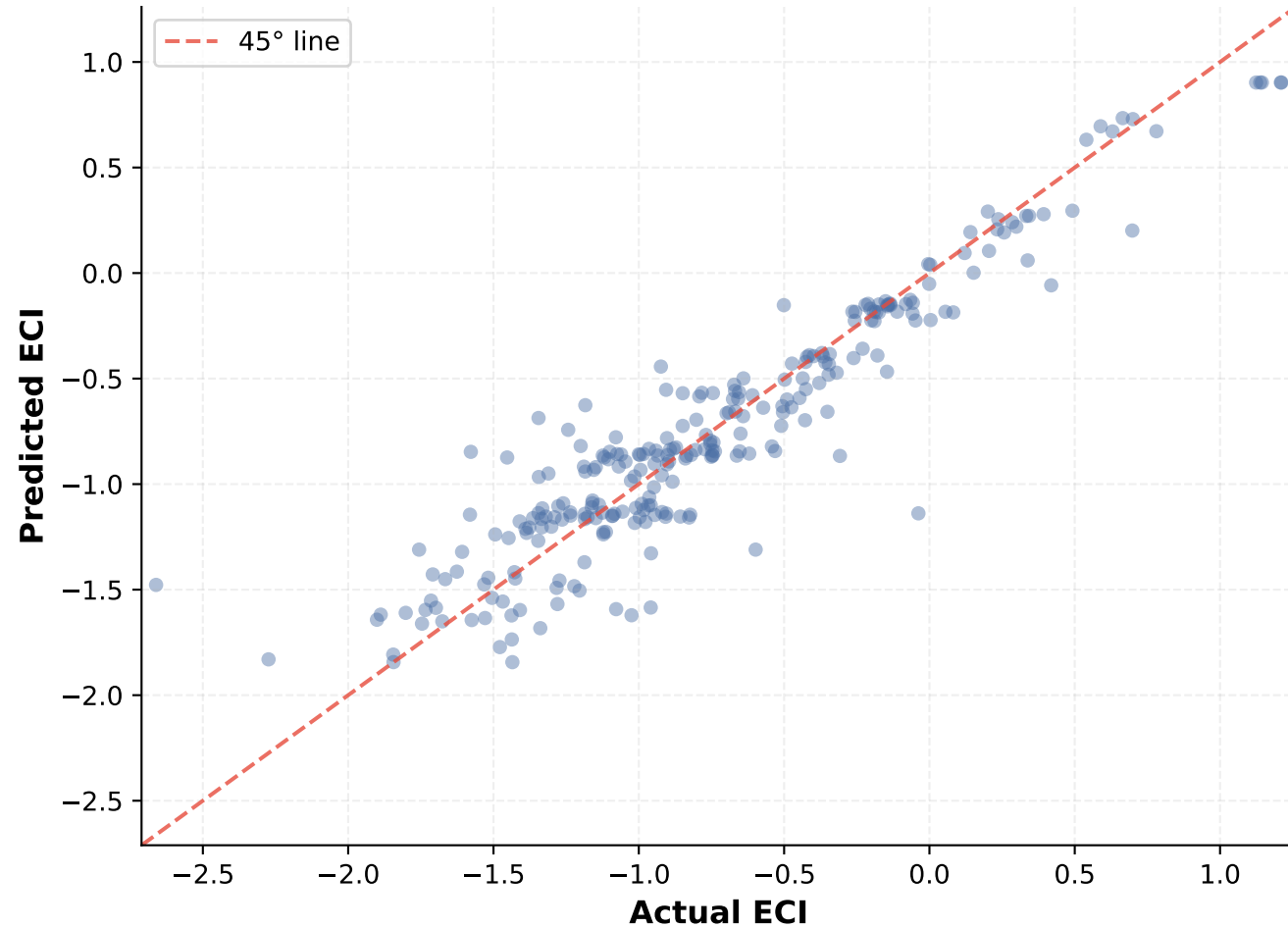
Random Forest — ECI Test R^2=0.874 | RMSE=0.2310
