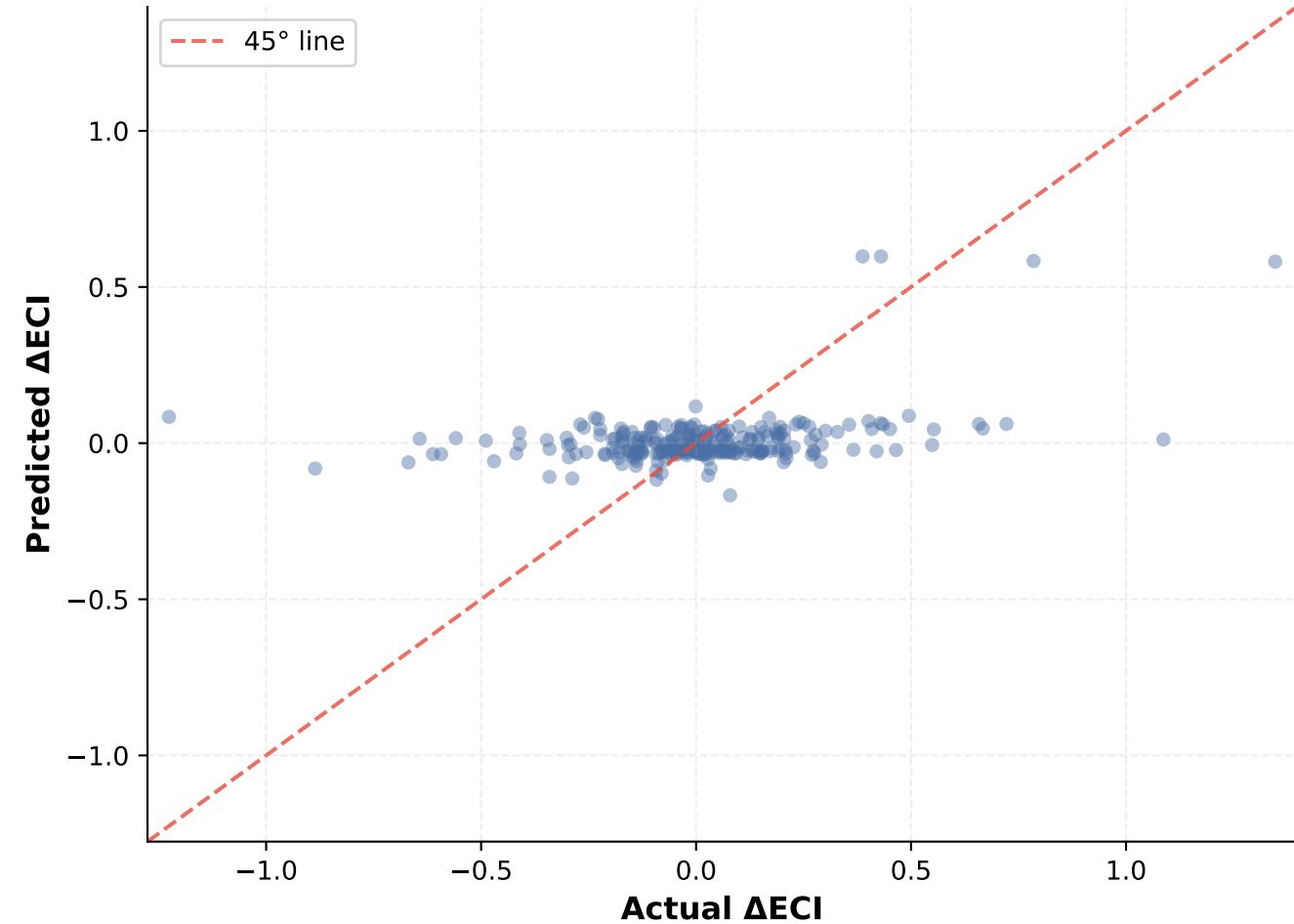
Random Forest — \Delta ECI Test R^2=0.150 | RMSE=0.2370
